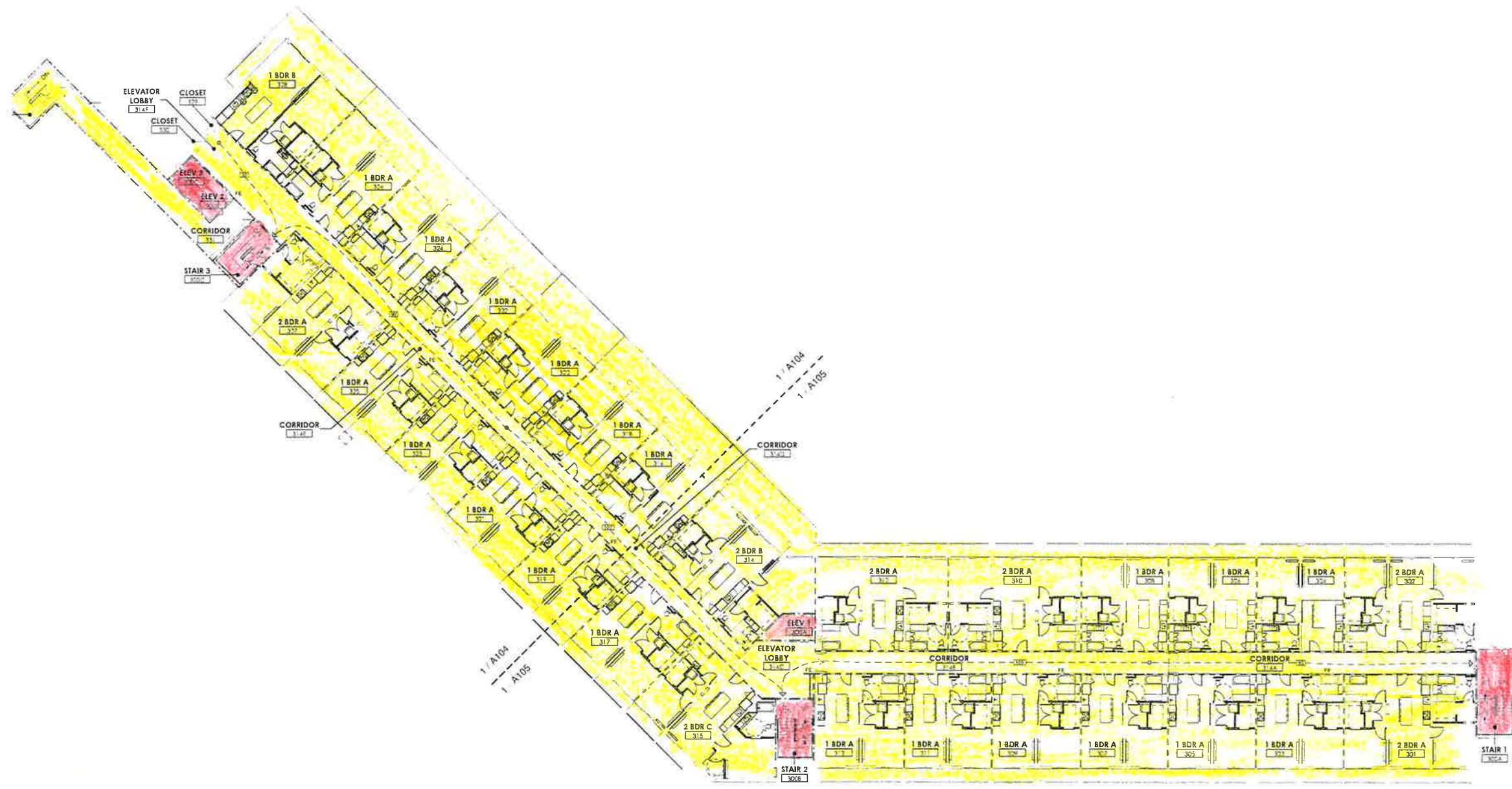
1 Third Floor Code Compliance Plan
