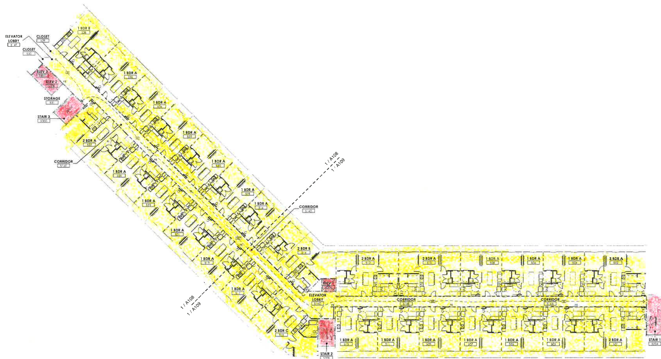
1 Fifth Floor Code Compliance Plan
