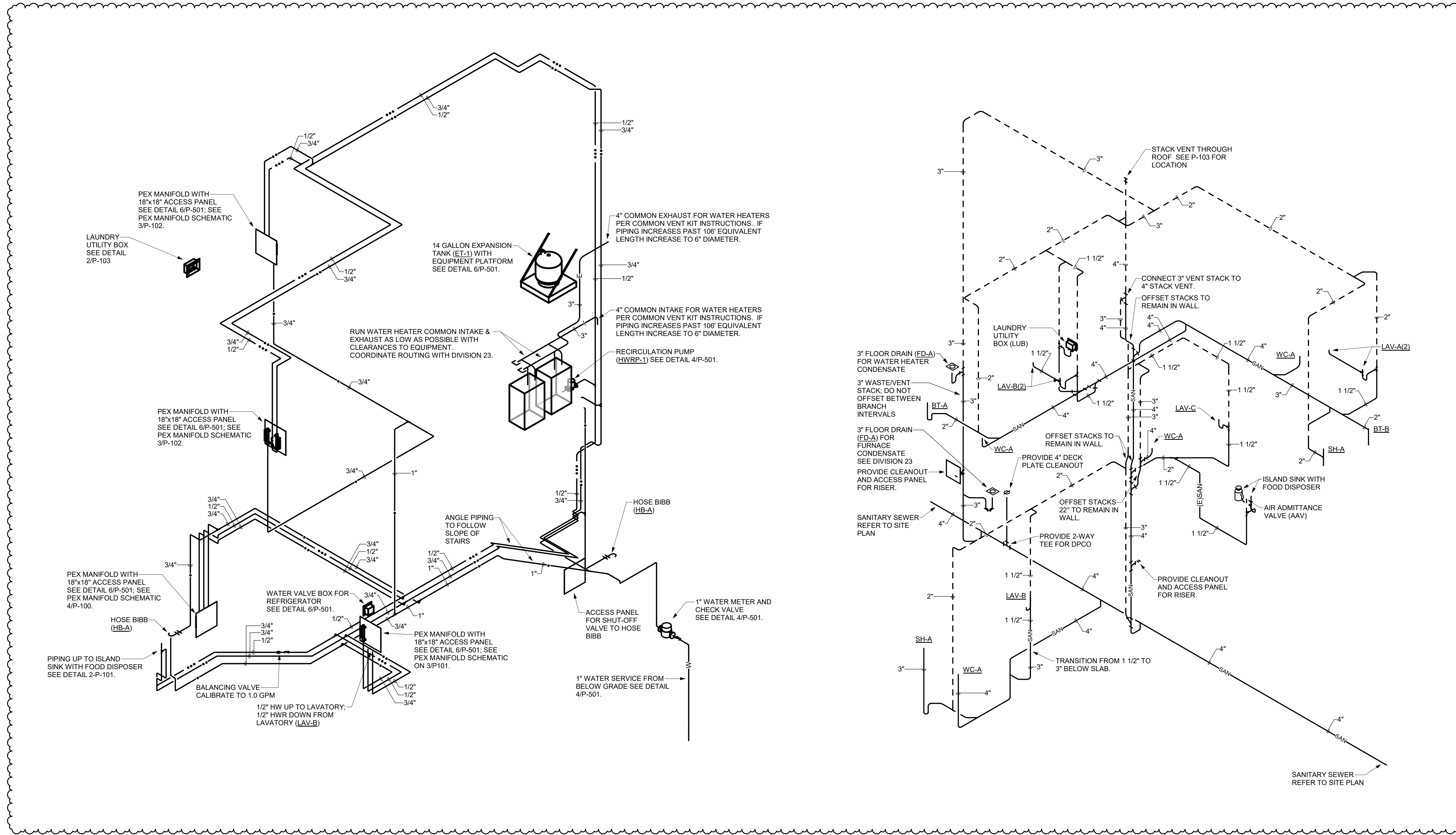
DOMESTIC WATER RISER DIAGRAM - PLUMBING
