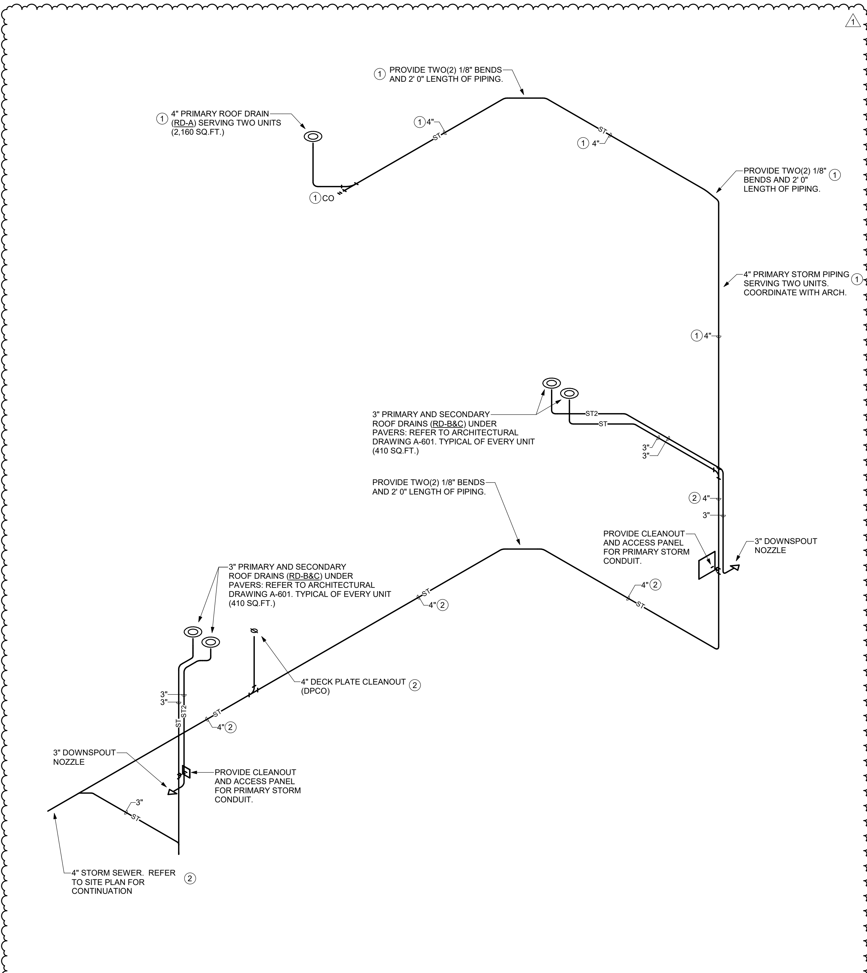
2 STORM RISER DIAGRAM - PLUMBING P-103
